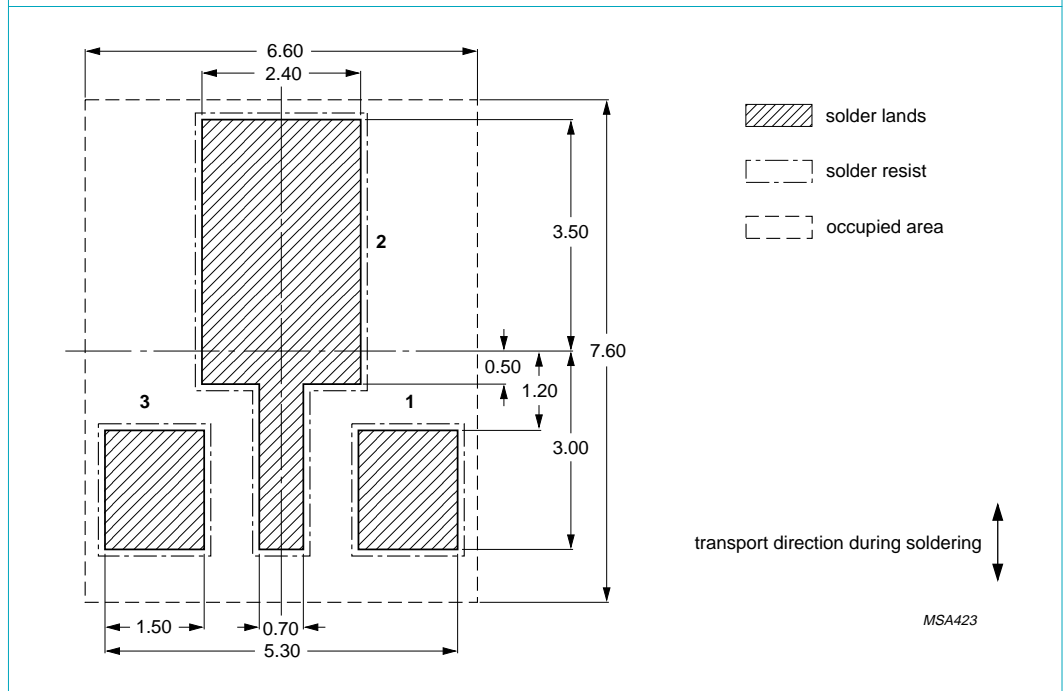
Not recommended for wave soldering Dimensions in mm
